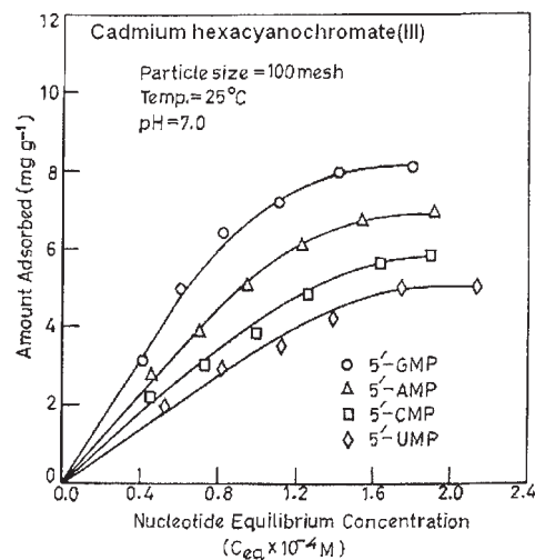
Fig. 4. Adsorption of ribonucleotides on cadmium(II) hexacyanochromate(III).
