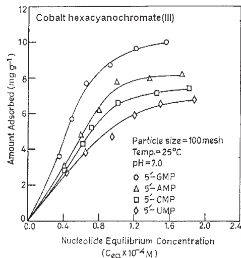
Fig. 3. Adsorption of ribonucleotides on cobalt(II) hexacyanochromate(III).
