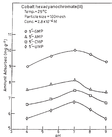
Fig. 1. Adsorption of ribonucleotides on cobalt(II) hexacyanochromate(III) as a function of pH.
