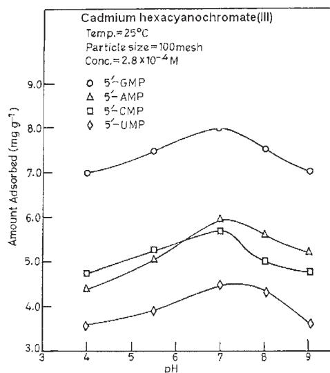
Fig. 2. Adsorption of ribonucleotides on cadmium(II) hexacyanochromate(III) as a function of pH.
